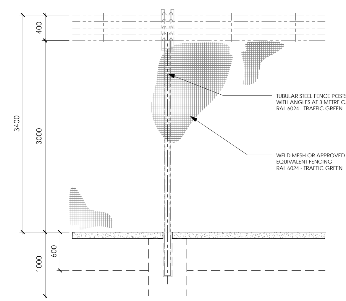
2 Security Fence NTS
