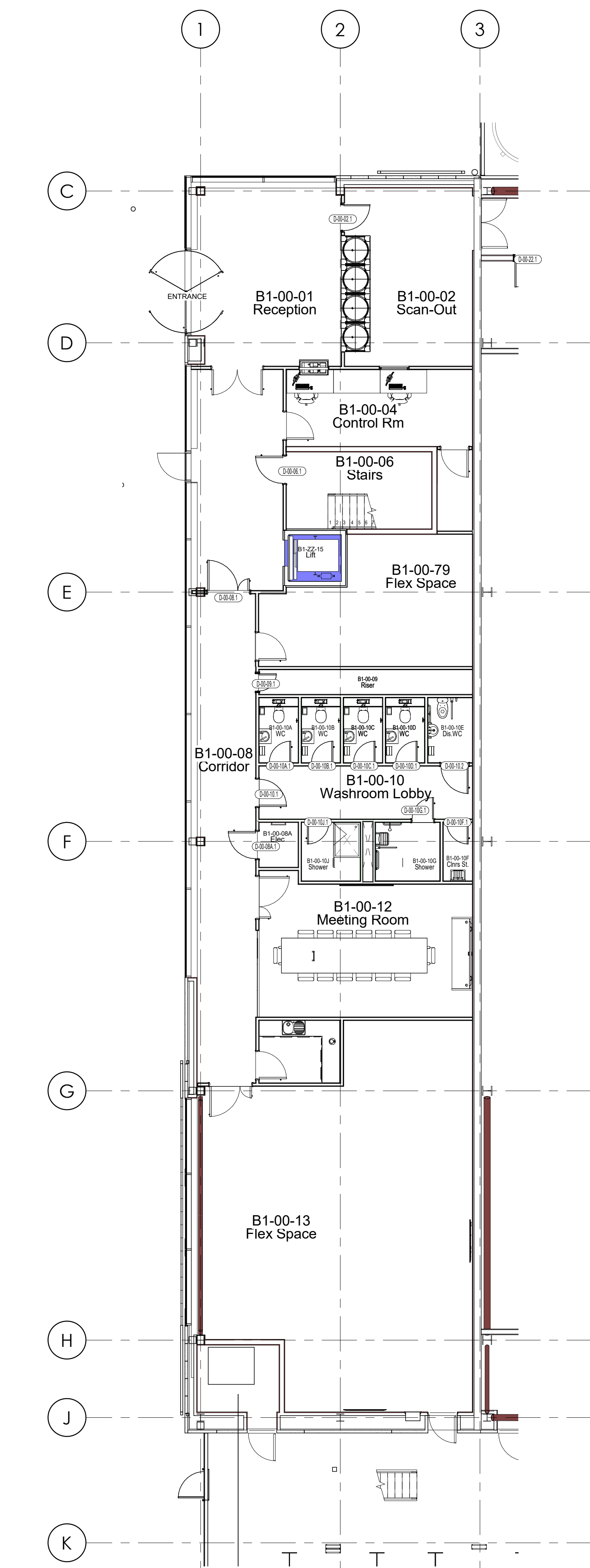
1 Level 00 - Office-Ground Floor 1:100
